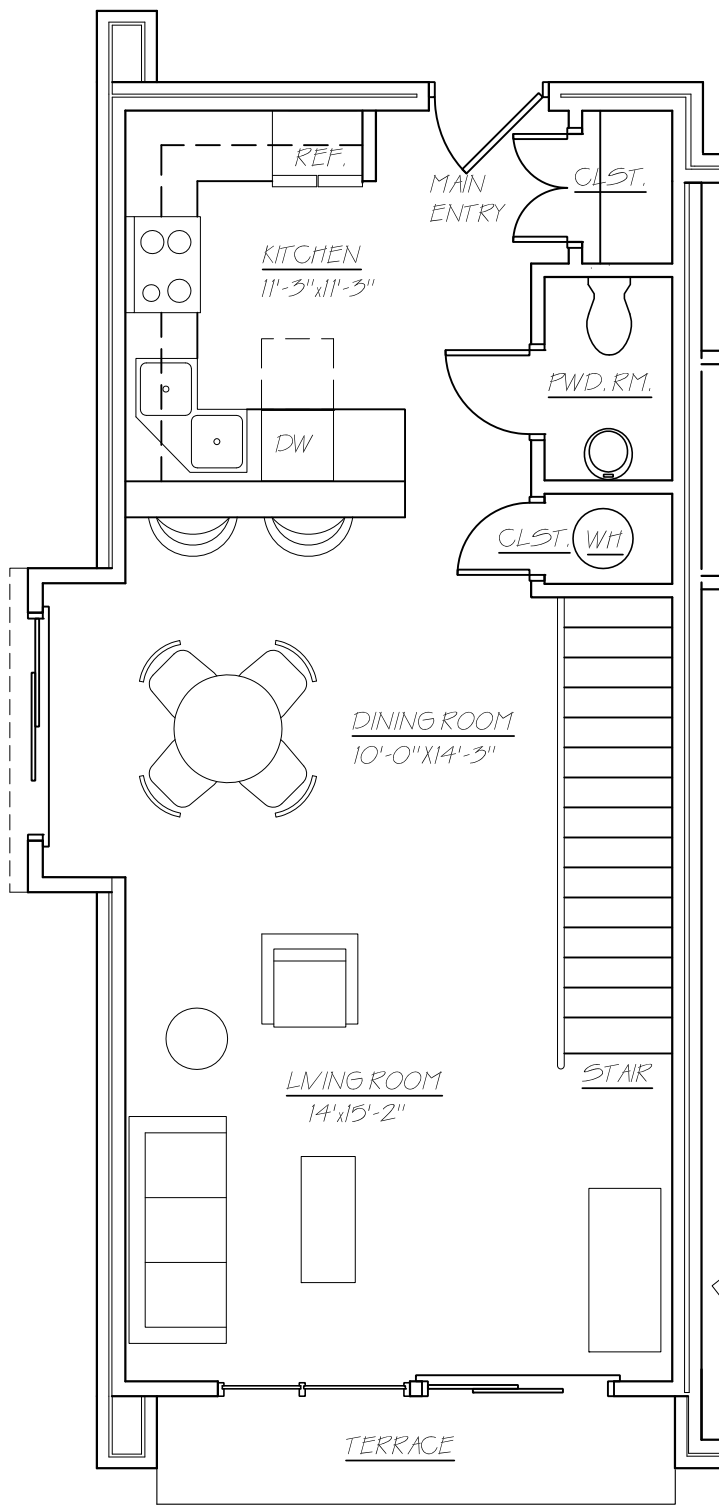
FIRST LEVEL
